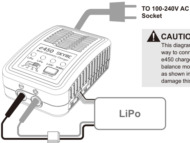
CONNECTION DIAGRAM
